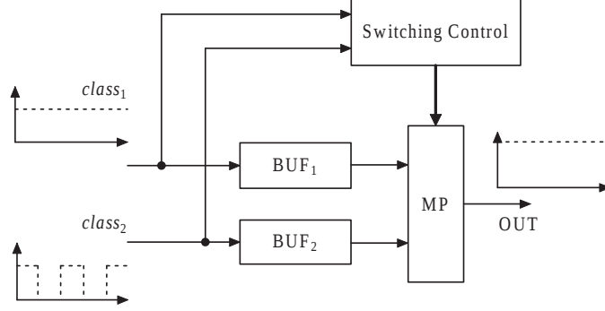
Figure I.1. Multiplexer scheme
