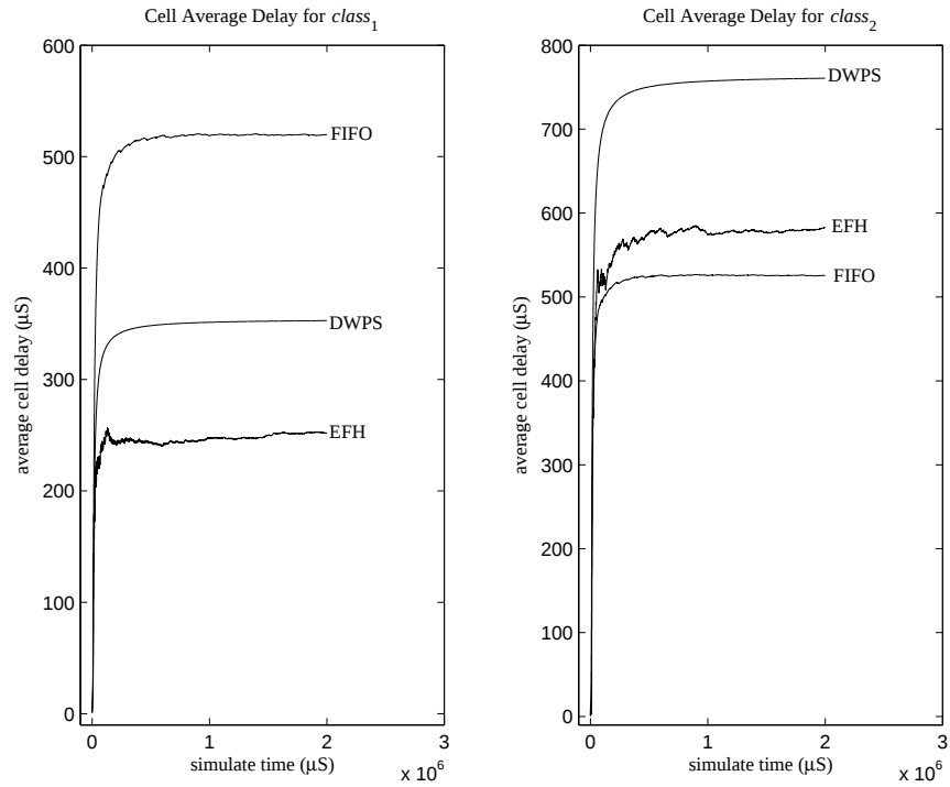
Figure I.8. Cell delay for class_1 and class_2 in scenario_2
