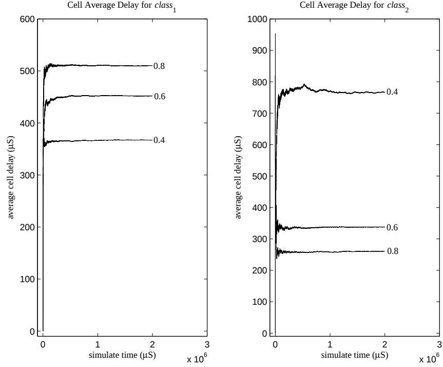
Figure I.10. Cell delay for scenario_1
