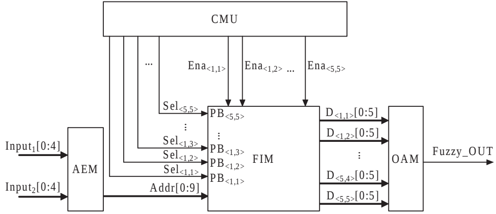
Figure I.14. Block architecture of RFIC
