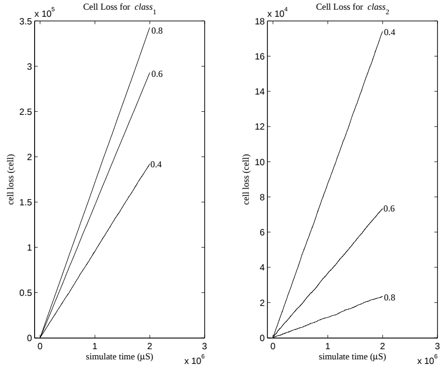
Figure I.11. Cell loss for scenario_1
