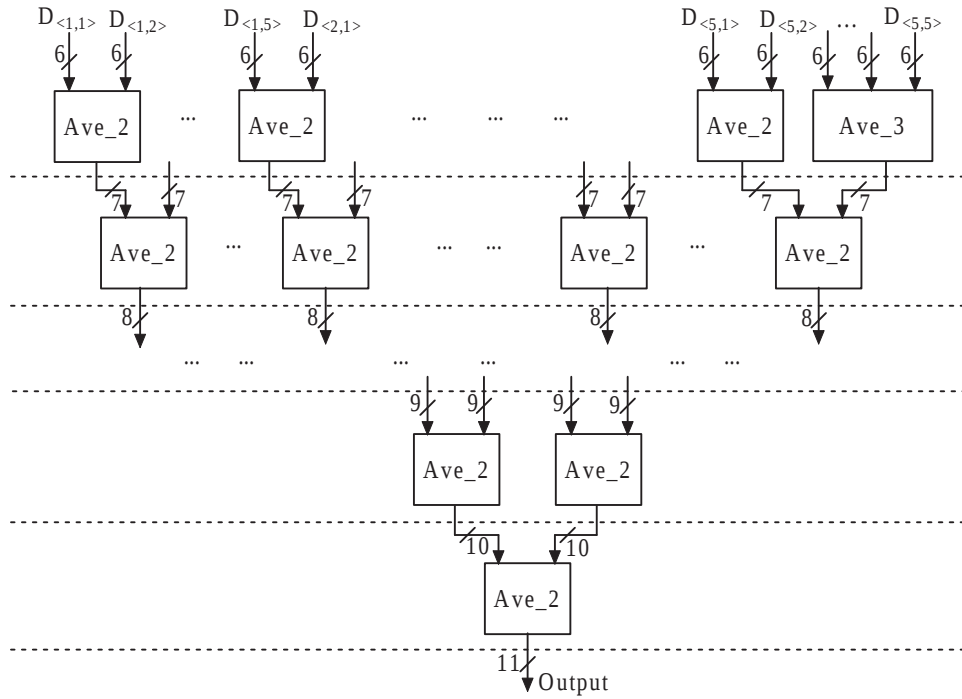
Figure I.15. The hardware architecture of OAM
