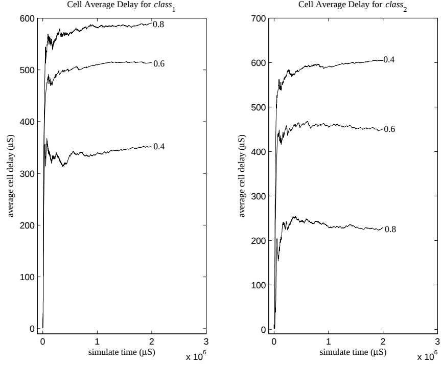
Figure I.12. Cell delay for scenario 2
