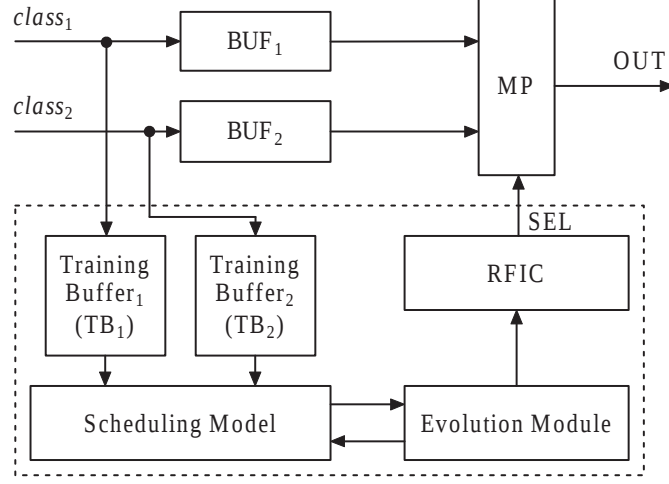
Figure I.2. Adaptation framework for EFH
