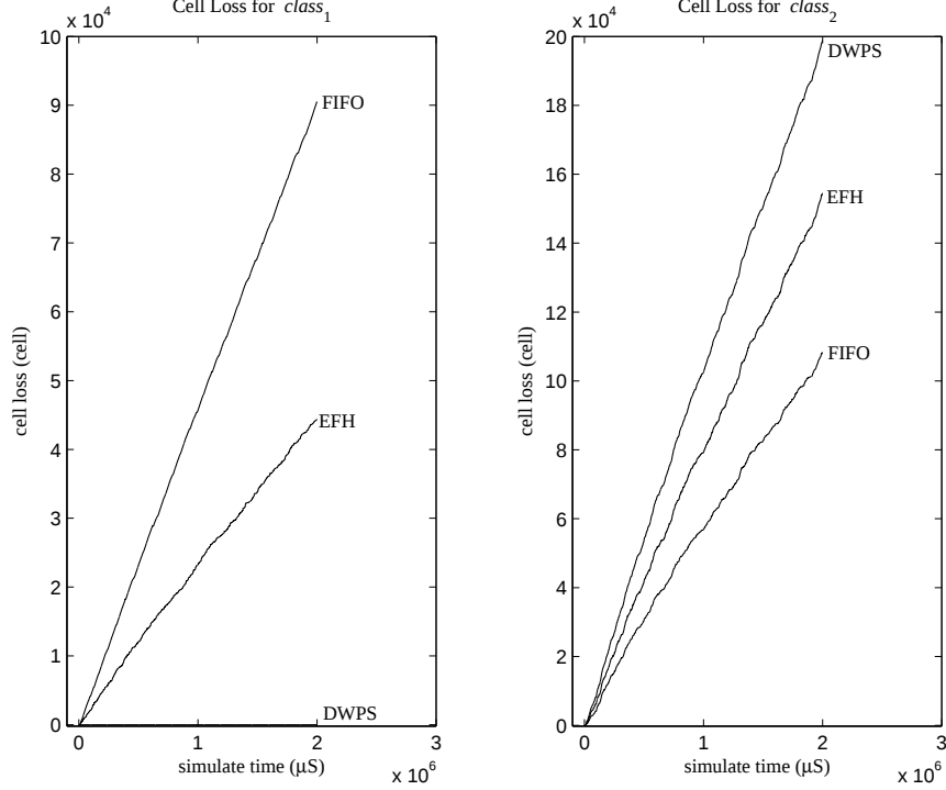
Figure I.9. Cell loss for class_1 and class_2 in scenario_2
