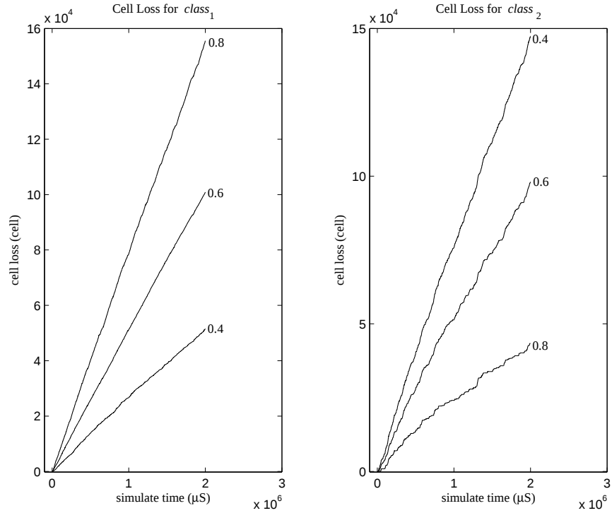
Figure I.13. Cell loss for scenario 2
