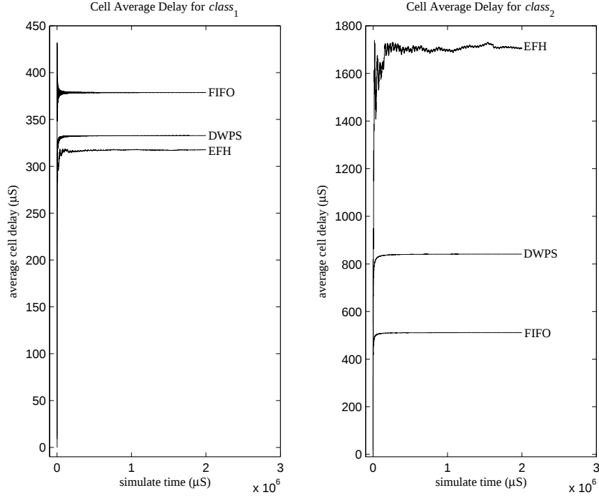
Figure I.6. Cell delay for class 1 and class 2 in scenario 1
