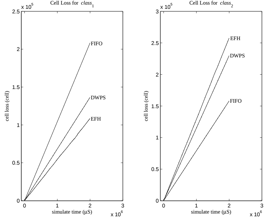
Figure I.7. Cell loss for class_1 and class_2 in scenario_1
