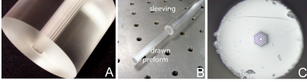
Figure 3. Three stages of MPOF manufacture.
